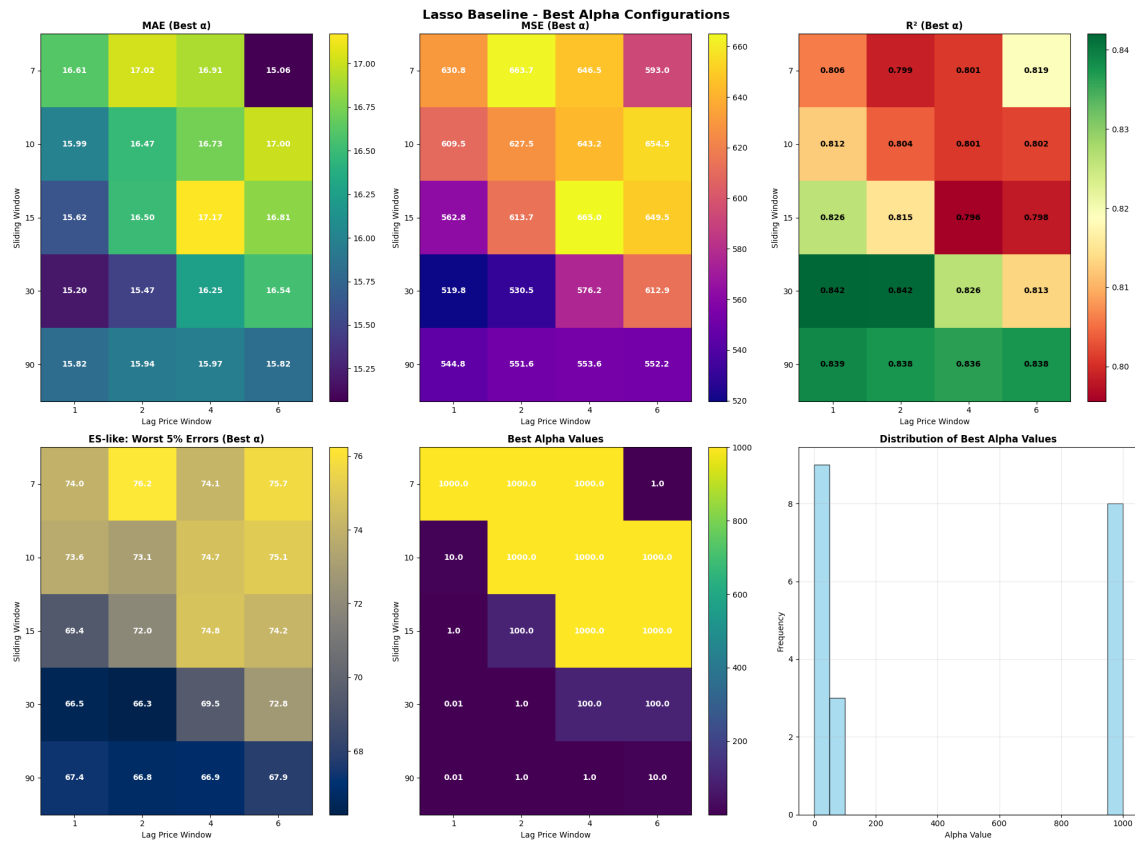
Fig. 4.12. Feature Engineering Lasso Best Alpha Metrics Distribution
